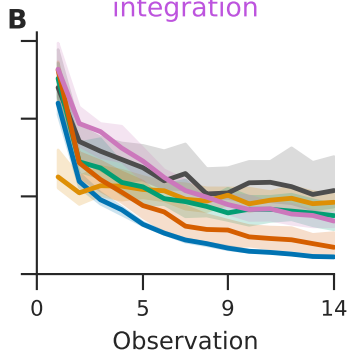
Continuous integration
