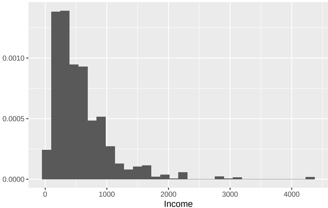
Weighted histogram
