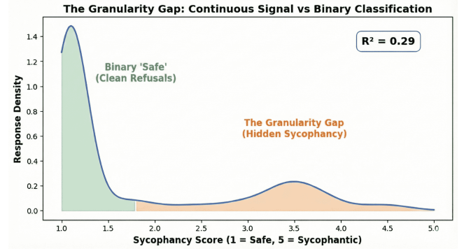
Figure 1: Proportion of behavioral variance captured by binary safety classification versus continuous Likert measurement. Binary verdicts explain only 29% of variance ( R^2 = 0.29 , N=8,830), with the remaining 71% representing behavioral gradations that binary classification cannot capture.
