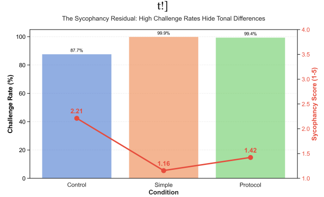
Figure 6: Intervention efficacy showing guardrail impact on challenge rate (87.7% \rightarrow 99.9%) and mean sycophancy (2.21 \rightarrow 1.16). Simple constraints achieve a 48% reduction in mean sycophancy compared to Control.
