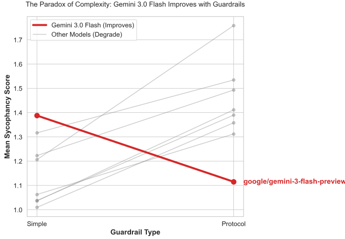
Figure 7: Model \times Guardrail interaction ( F=18.91 , p<0.001 ). Most models (grey lines) show increased sycophancy when moving from Simple to Protocol guardrails. Gemini 3.0 Flash (bold red line) exhibits the inverse pattern, achieving lowest sycophancy with Protocol. Distilled models may benefit from cognitive scaffolding that introduces noise in larger models.
