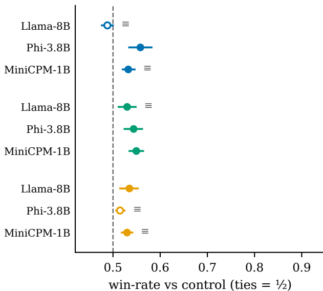
Fine-tuning (lora vs base): 7/9 Holm
