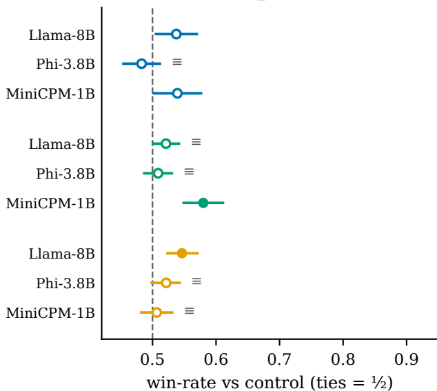
RAFT synergy (lora_rag vs rag): 2/9 Holm
