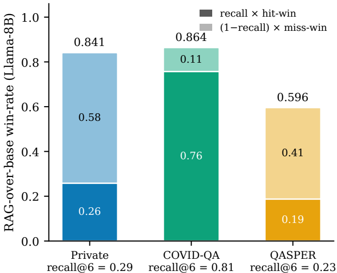
(a) Decomposition of the retrieval effect
