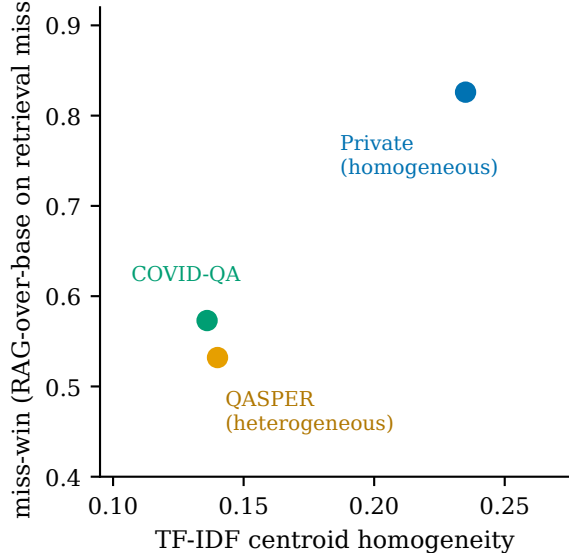
(b) Homogeneity vs miss-win
