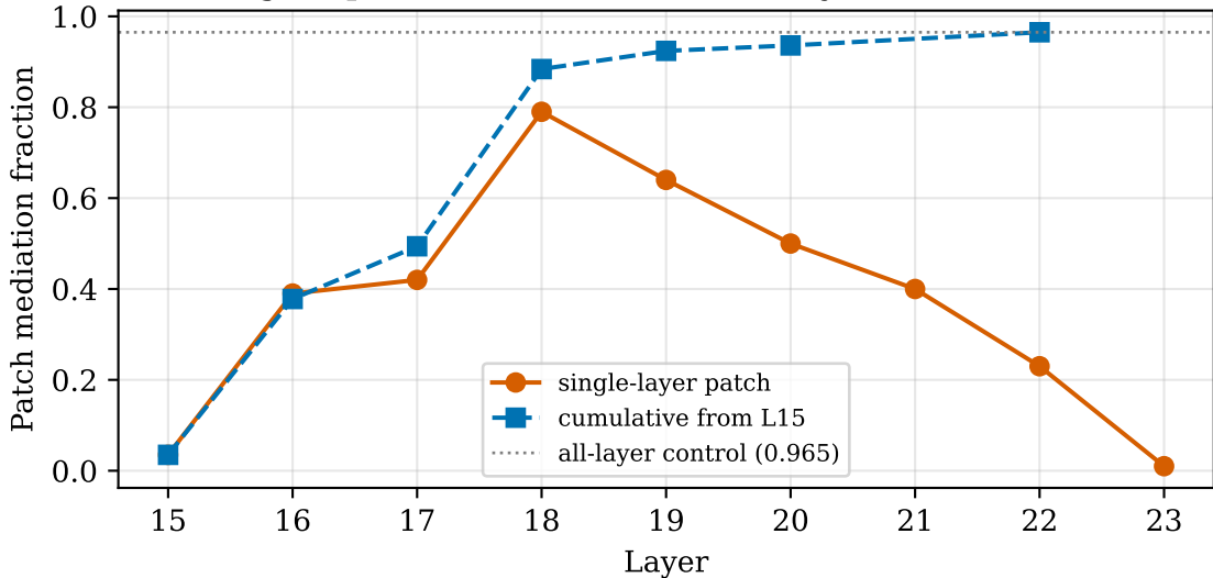
SES signal patchable in a narrow early band (Qwen suffix)
