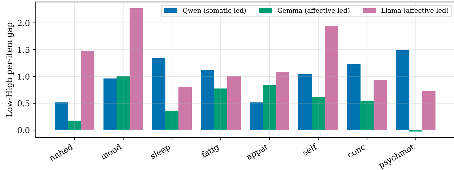
Stereotype content differs by model (PHQ-8 item decomposition, all 3 models)
