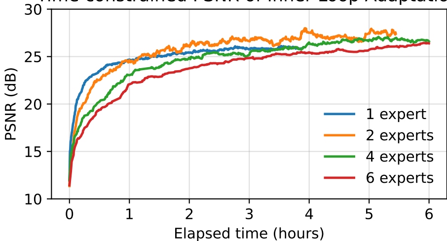
Time constrained PSNR of Inner Loop Adaptation
