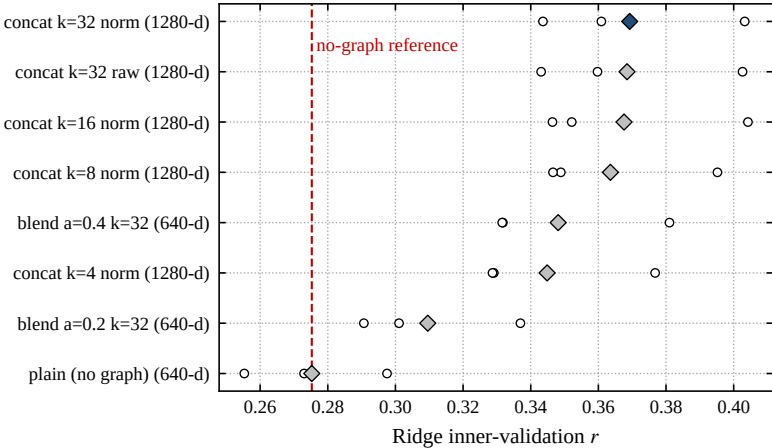
(a) Ridge readout (diamond = mean of 3 splits, circles = splits)
