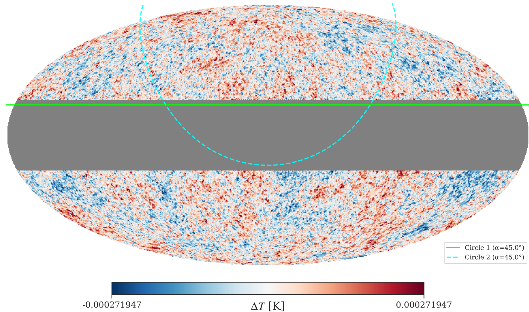
CMB with Best Matched Circles
