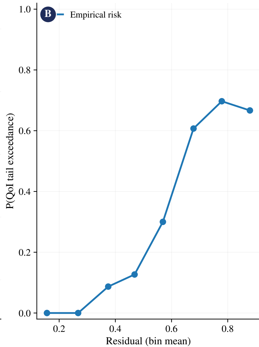
Residual-to-risk calibration
