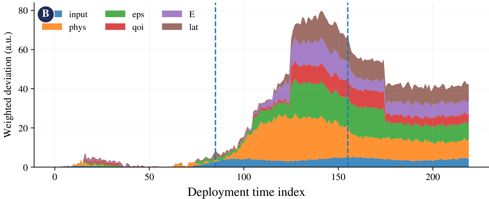
Decomposable diagnosis via dominant contributors
