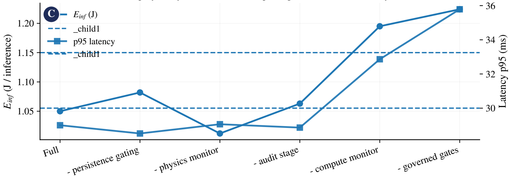
Deployability failure modes (compute+governance are necessary)
