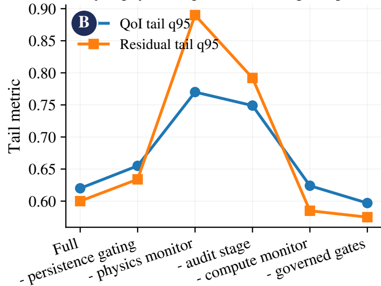
Deployability failure modes (compute+governance are necessary)
