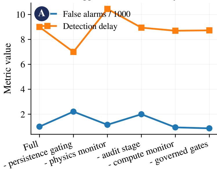
Deployability failure modes (compute+governance are necessary)
