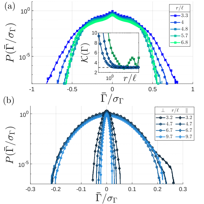
FIG. 3: PDFs of the velocity circulation for different loop sizes r/\ell > 1 , scaled by the standard deviation \sigma_\Gamma . (a) shows the Taylor-Green simulation, while (b) shows both of the normal fluid parallel (diamonds) and perpendicular (circles) components. The inset of (a) shows the flatness \mathcal{K}(\Gamma) = \langle |\Gamma|^4 \rangle / \sigma_\Gamma^4 , with the same color scheme as in Fig. 2. The black dashed line marks the Gaussian flatness of \mathcal{K} = 3 . See the Supplementary materials for the SF PDFs.
