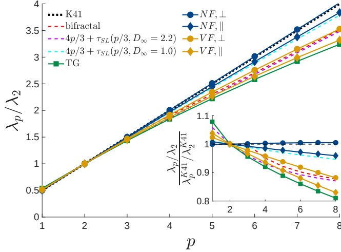
FIG. 5: Scaling exponents of velocity circulation moments, estimated within the classical range r > \ell . The colour scheme and line styles is the same as in Fig. 2. The black dashed line represents the self-similar K41 scaling \lambda_p^{K41} = 4p/3 . The inset shows the proportional deviation from K41 theory.
