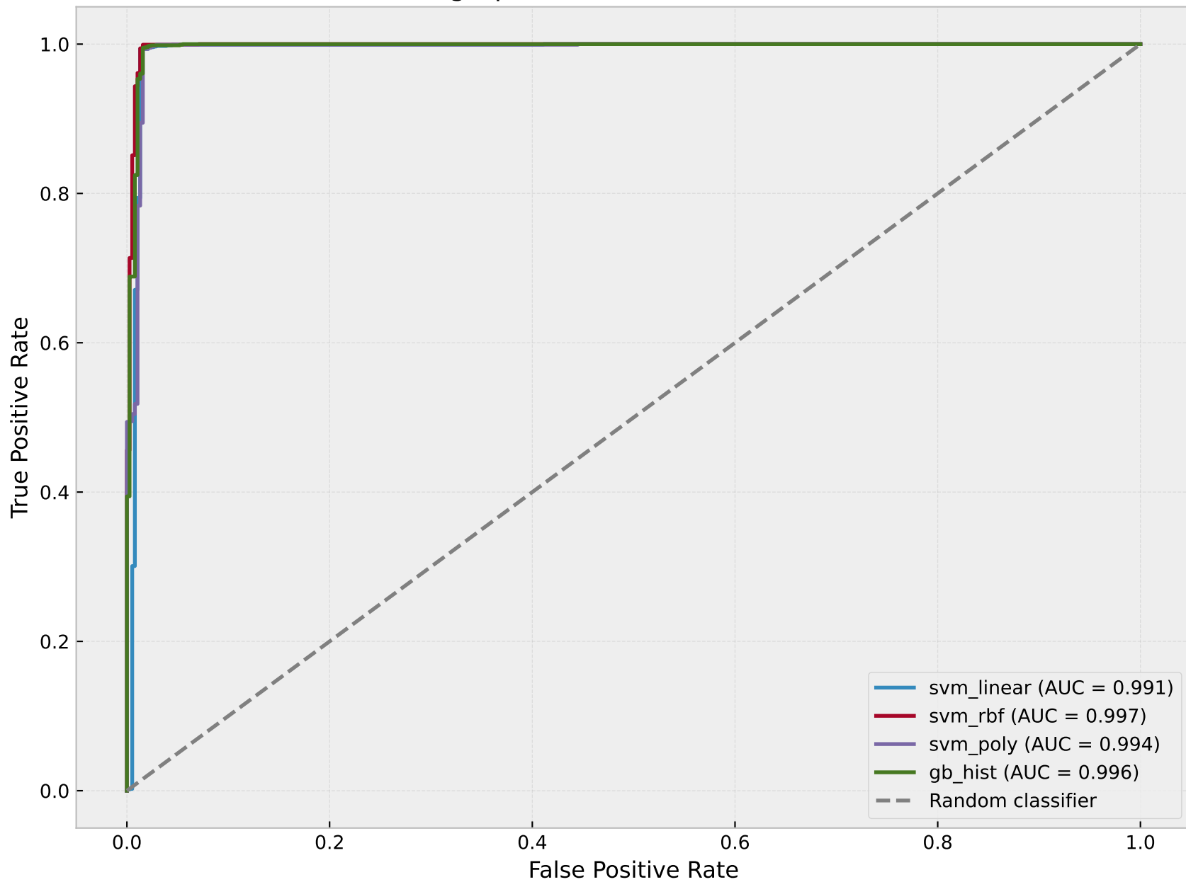
ROC-graphs for different SVM kernels
