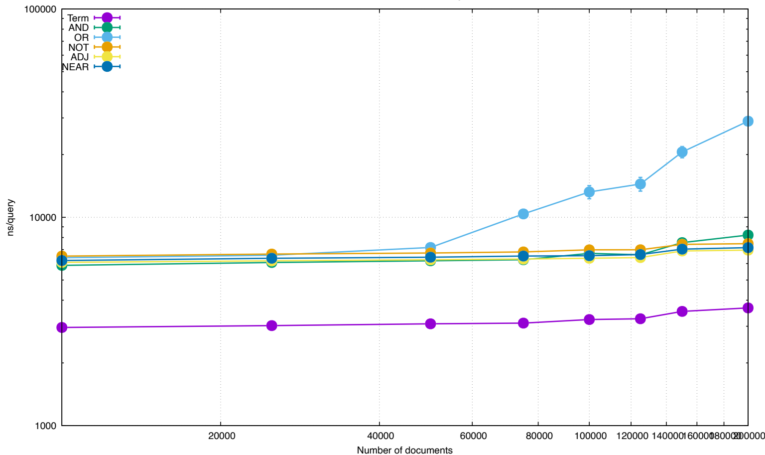
Query latency with ranking
