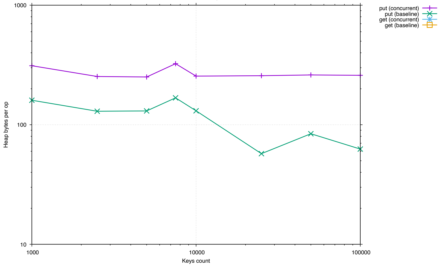
Memory per operation (single thread)
