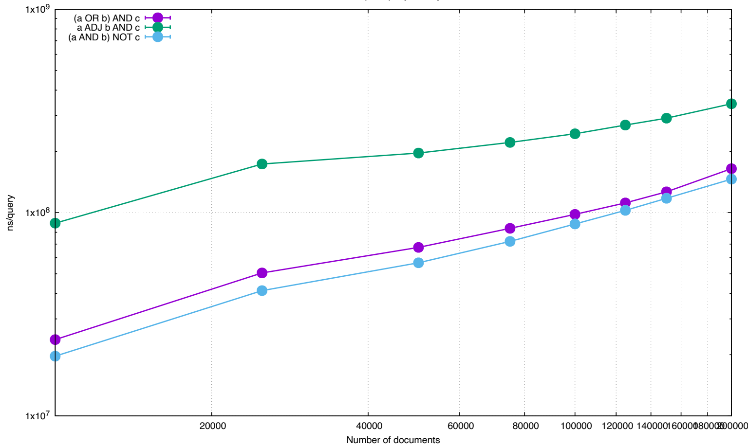
Complex query latency
