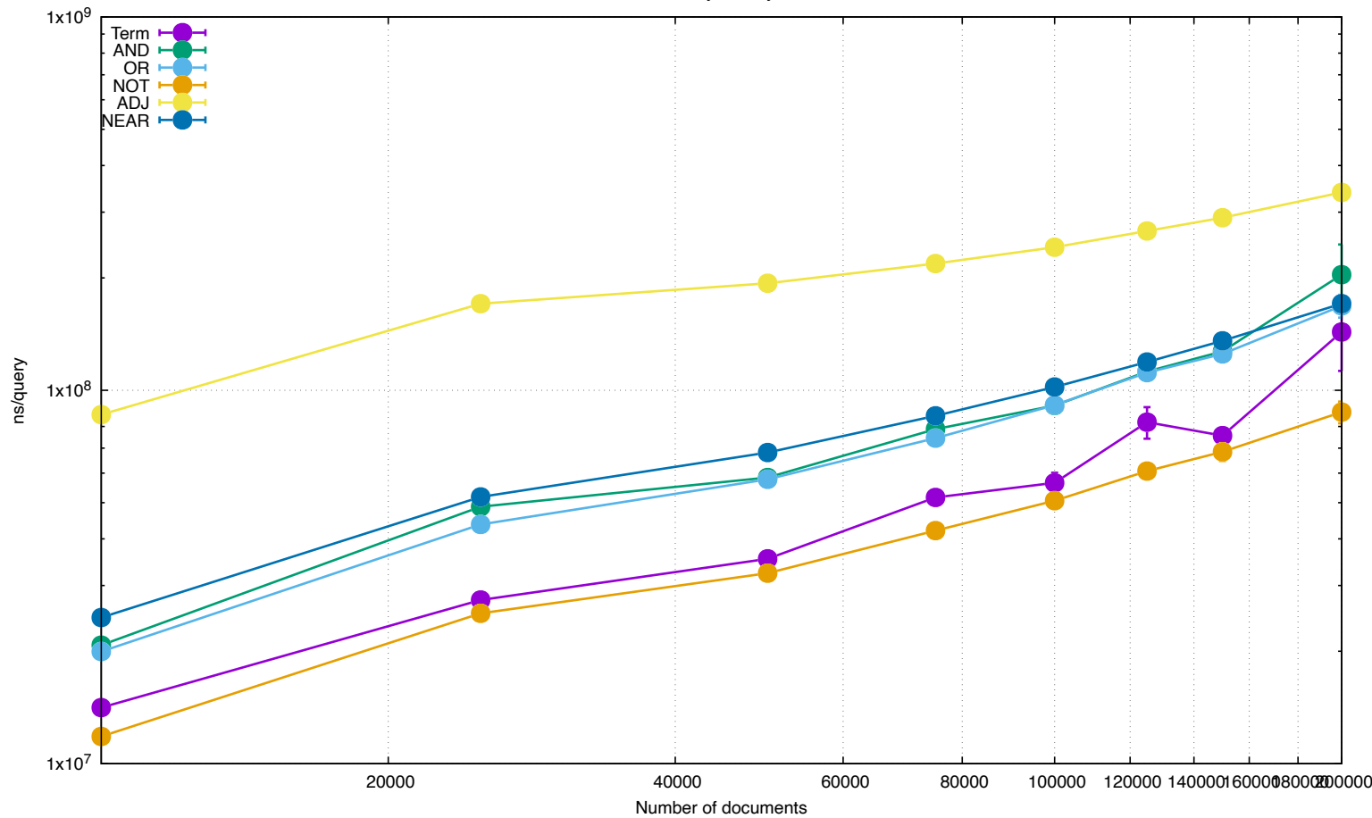
Query latency
