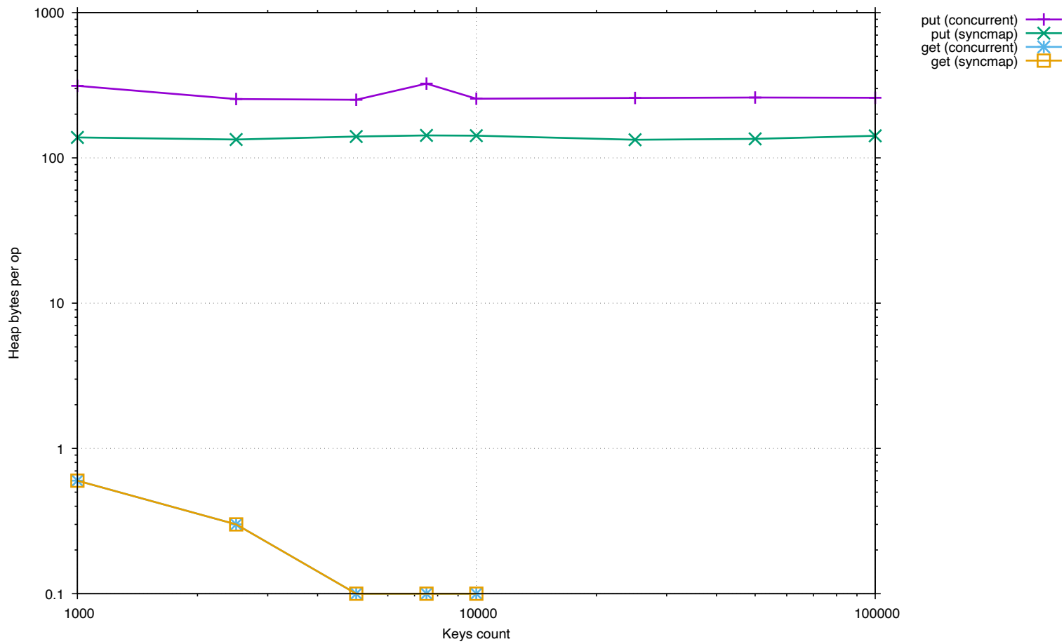
Memory per operation (multi thread)
