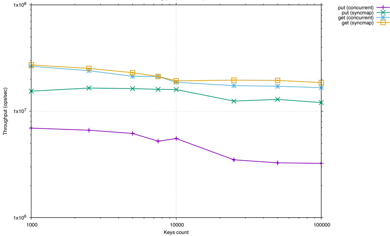
Throughput (multi thread)
