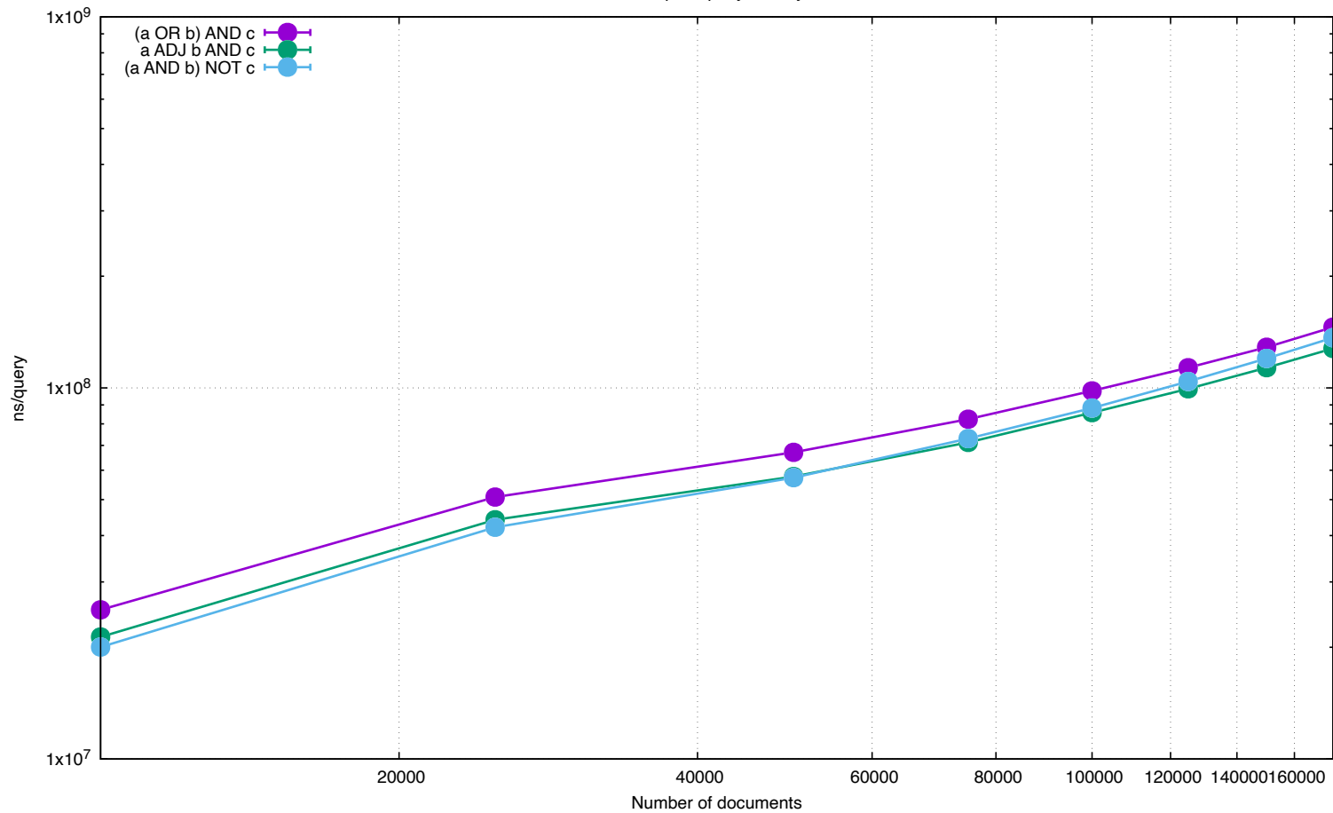
Complex query latency
