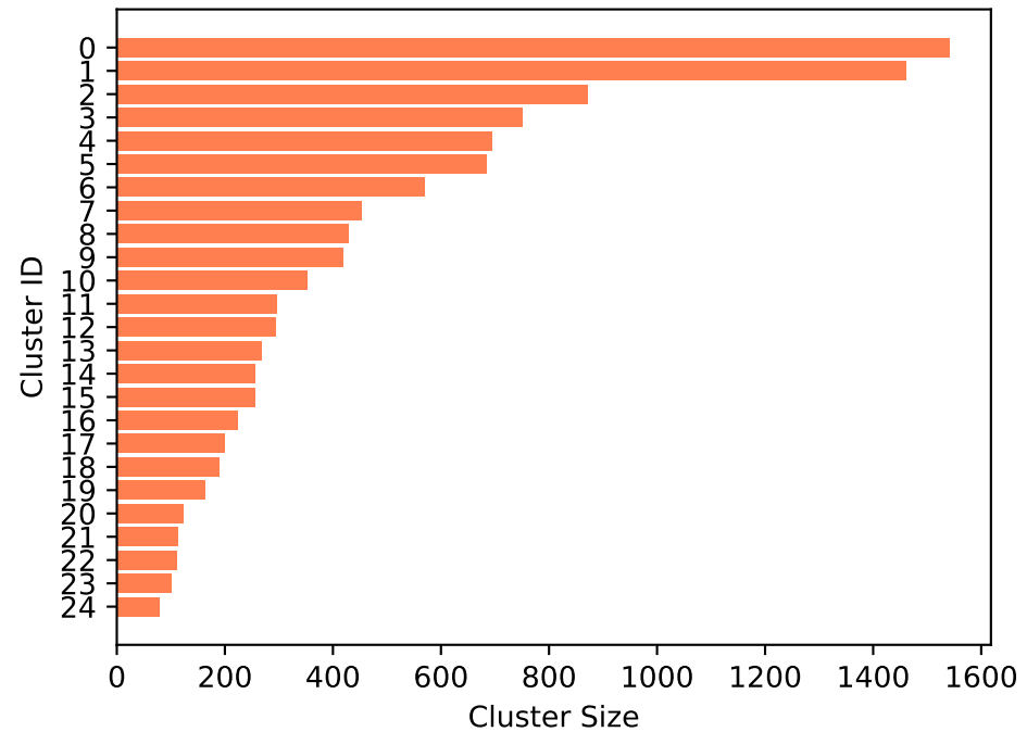
Top-25 Largest Clusters
