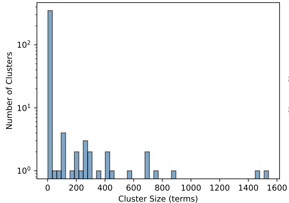
Cluster Size Distribution
