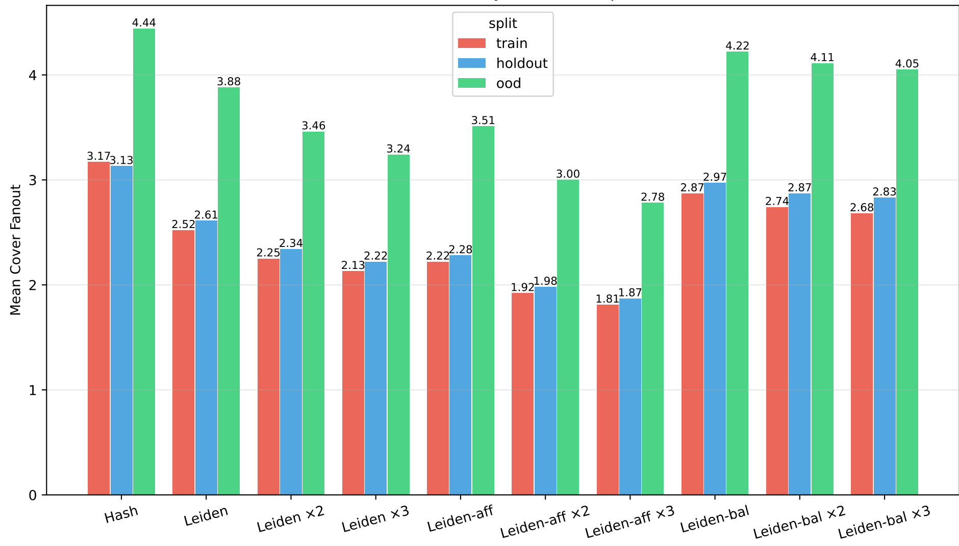
Cover Fanout by Evaluation Split
