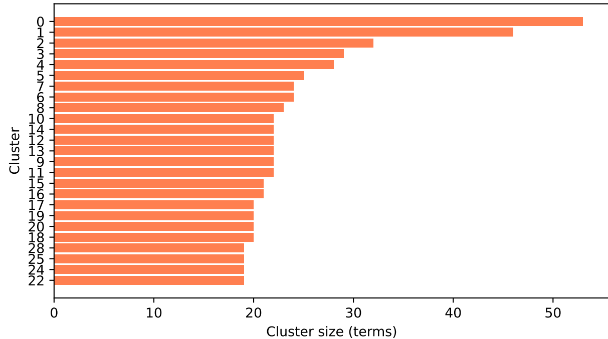
25 largest clusters
