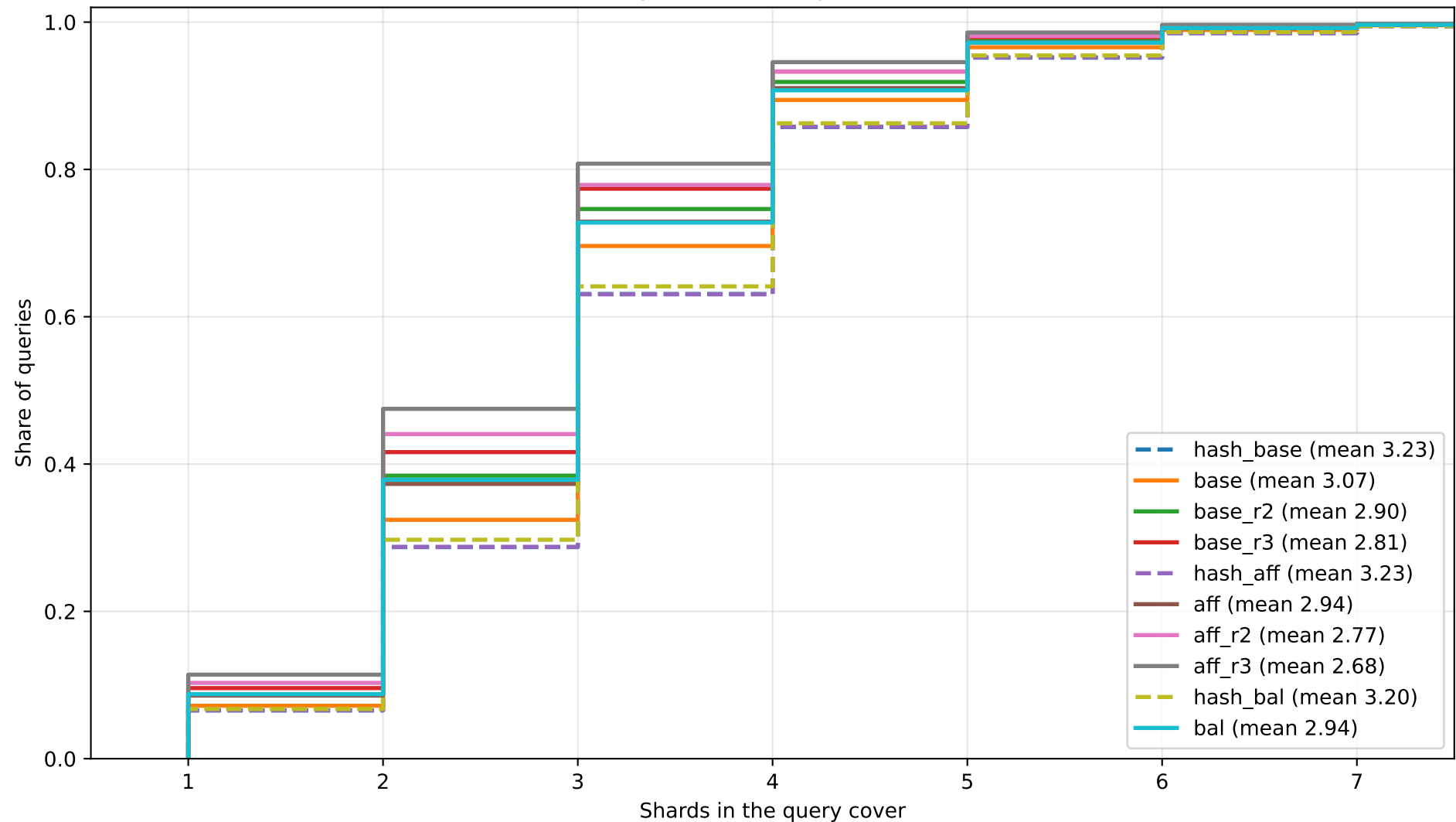
Query cover size: cpm, holdout
