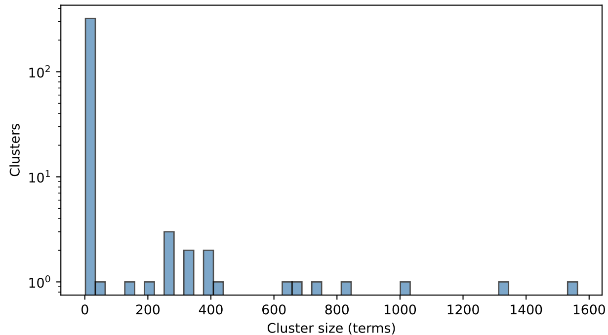
Cluster sizes: leiden
