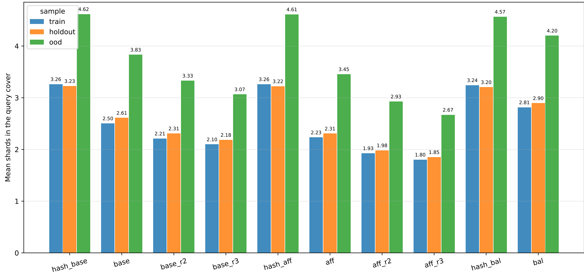
Query cover size by sample: leiden
