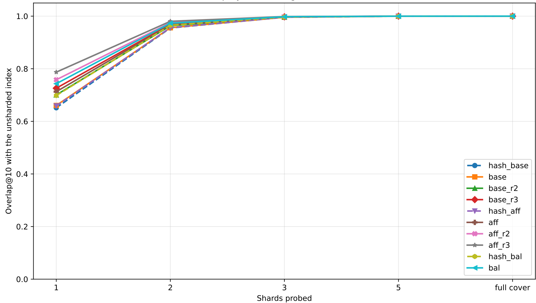
Overlap by shard budget: metis, holdout
