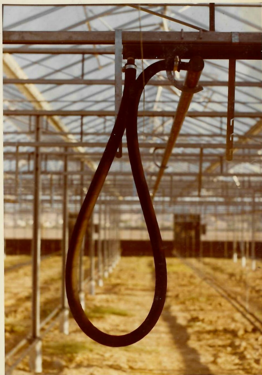
MOVEABLE HEATING SYSTEM SHOWN IN THE RAISED POSITION TO ALLOW FOR MORE WORKING ROOM ON THE FLOOR OF THE HOUSE
