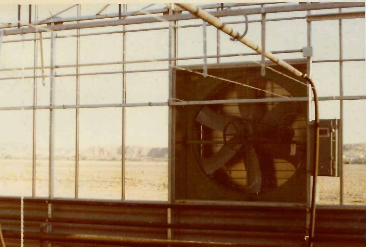
FAN AT OPPOSITE END OF HOUSE FROM THE EVAPORATIVE PAD TO DRAW AIR THROUGH THE BUILDING FOR THE COOLING SYSTEM
