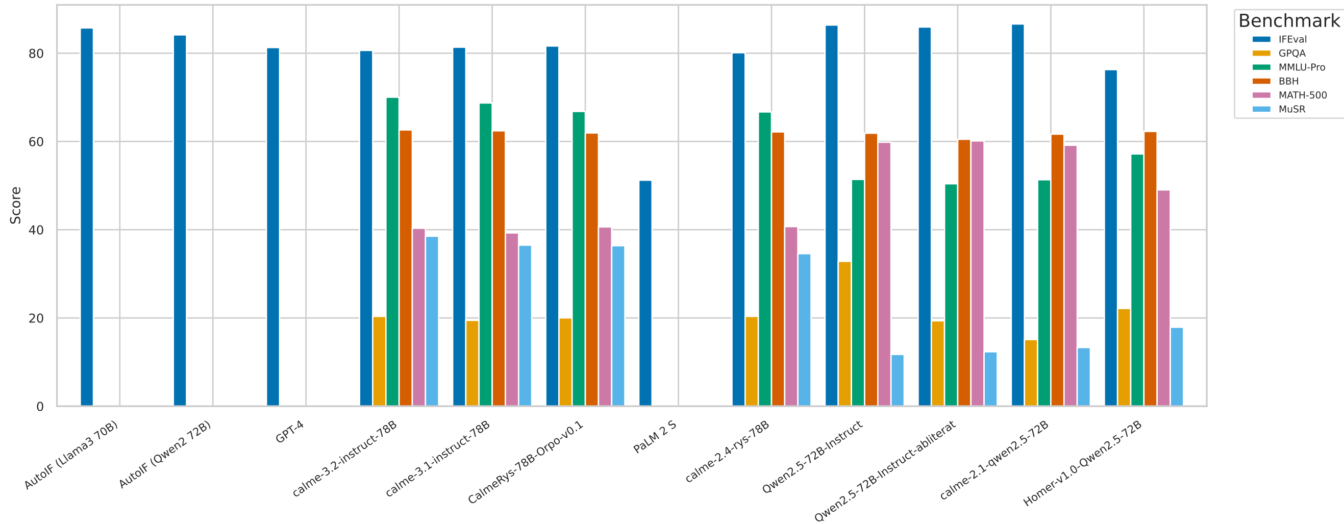
Top Models Across Open LLM Leaderboard v2 Benchmarks
