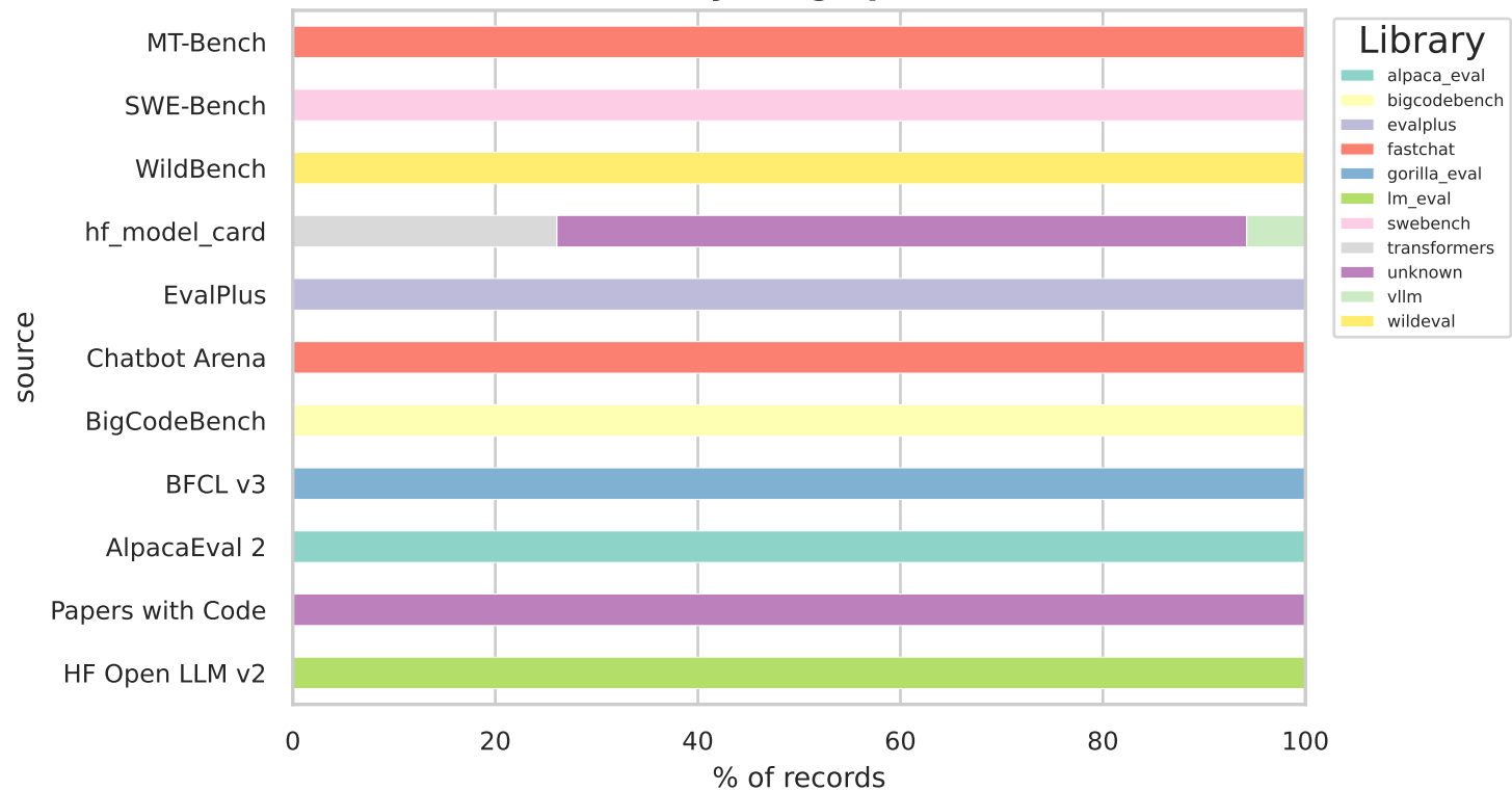
(b) Library usage per source
