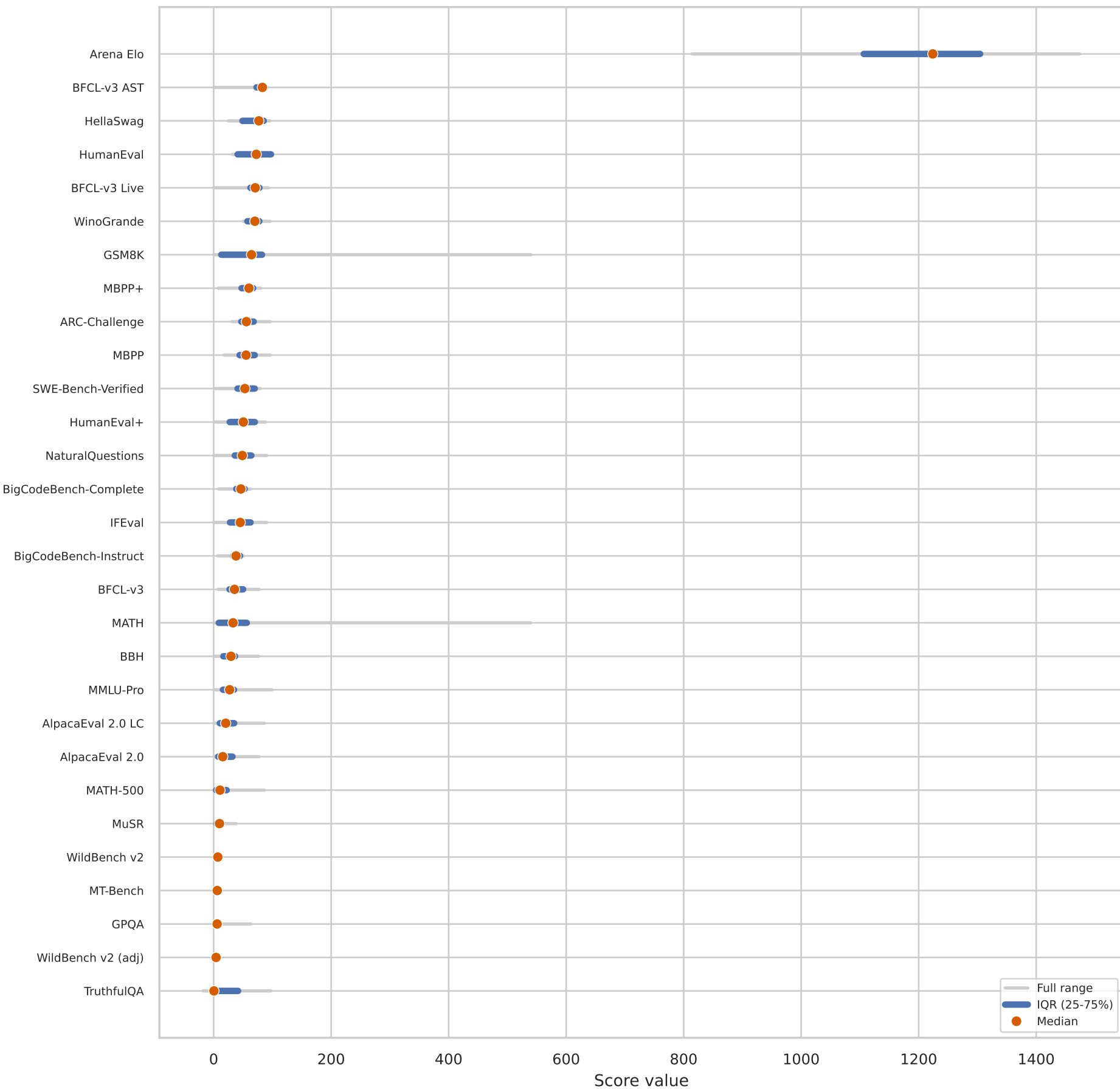
Score Scale Heterogeneity Across Benchmarks (grey = full range, blue = IQR, orange dot = median)
