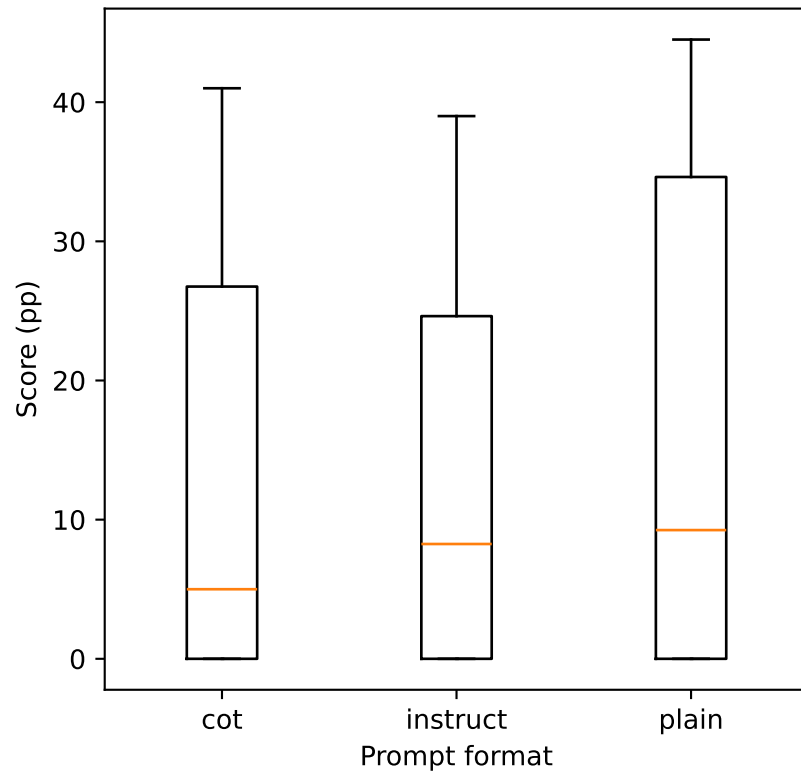
GSM8K scores by Prompt format
