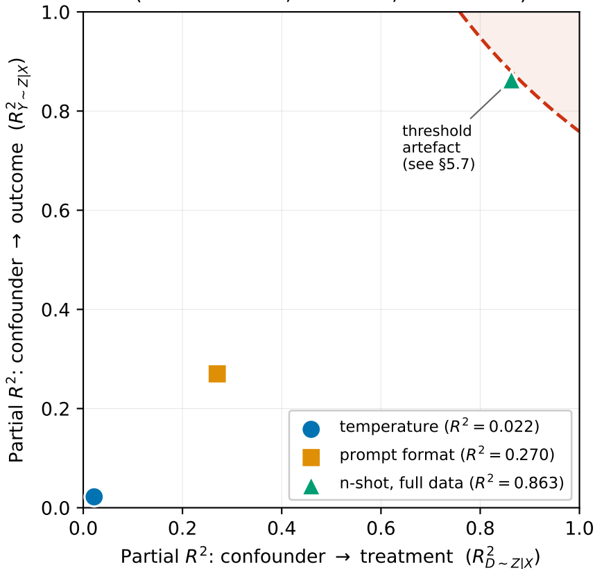
Cinelli-Hazlett sensitivity for \rho = -0.871 (5-shot GSM8K, 3 models, n = 54 runs)
