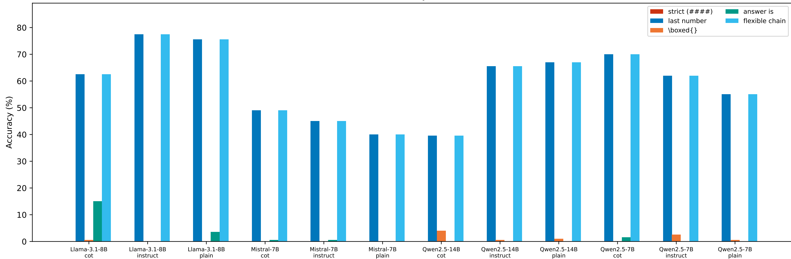
Cross-Extractor Study: 0-shot GSM8K
