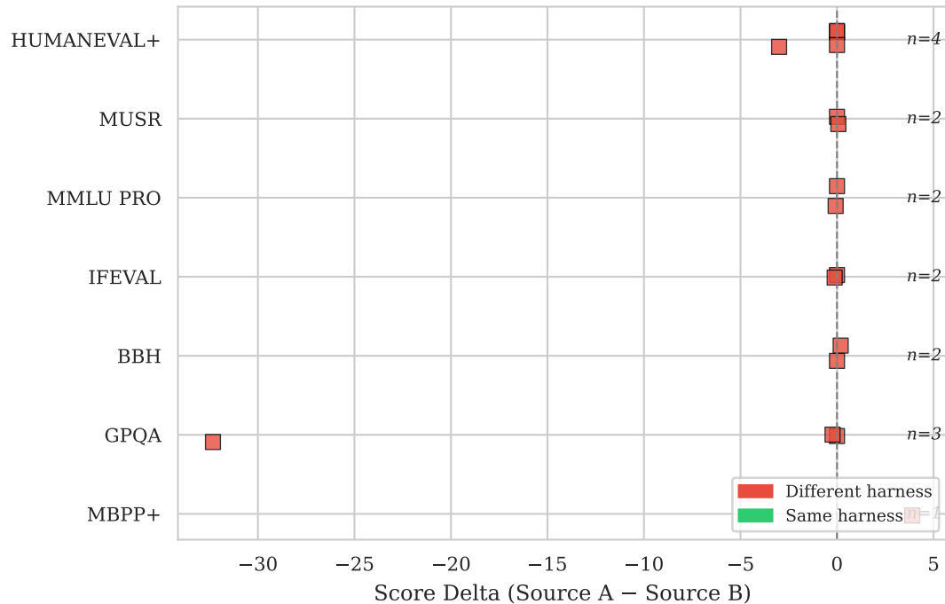
Cross-Source Score Differences
