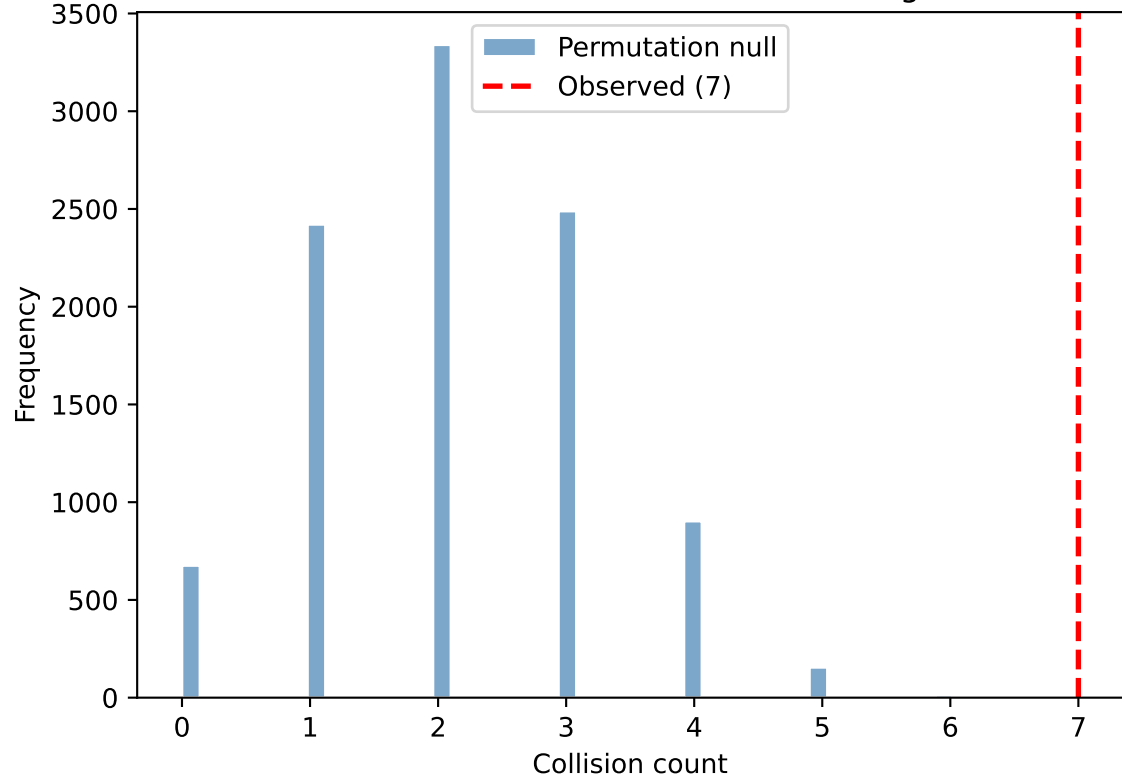
Permutation Null Distribution — Excluding OLv2
