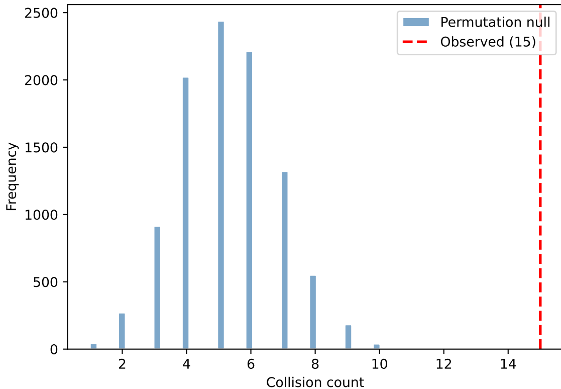
Permutation Null Distribution — All Sources
