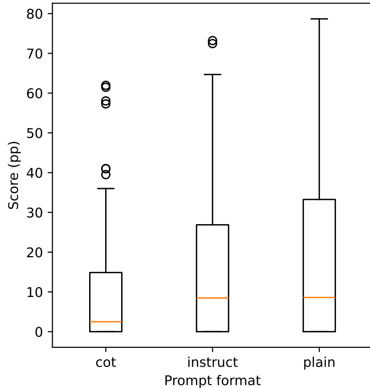
Score distribution by Prompt format
