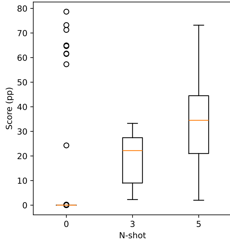
Score distribution by N-shot
