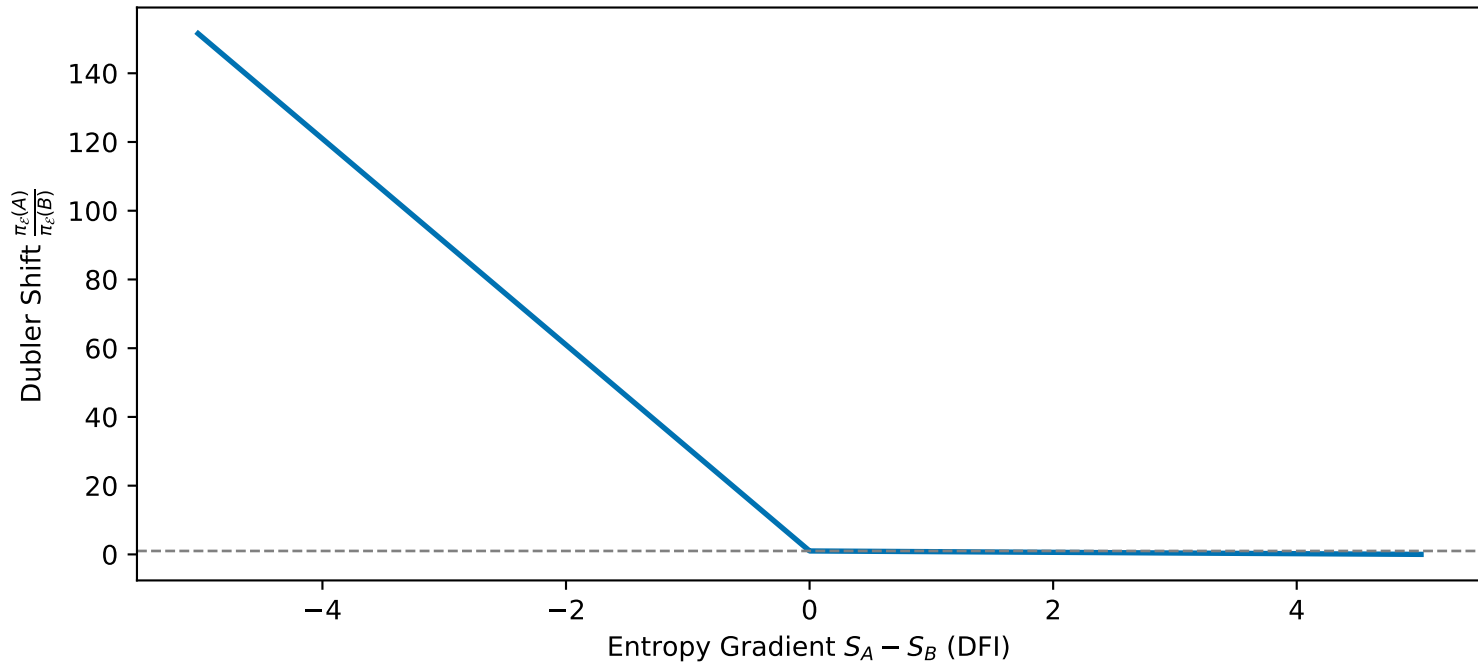
Generic Dubler Shift: DFI + Elastic \pi ( \mathcal{K}_D = 1 )
