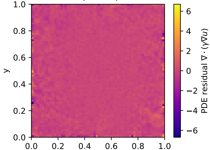
PDE Residual (Linear) for BC k=20
