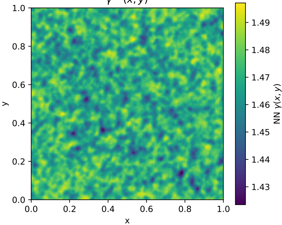
\gamma^{NN}(x, y)
