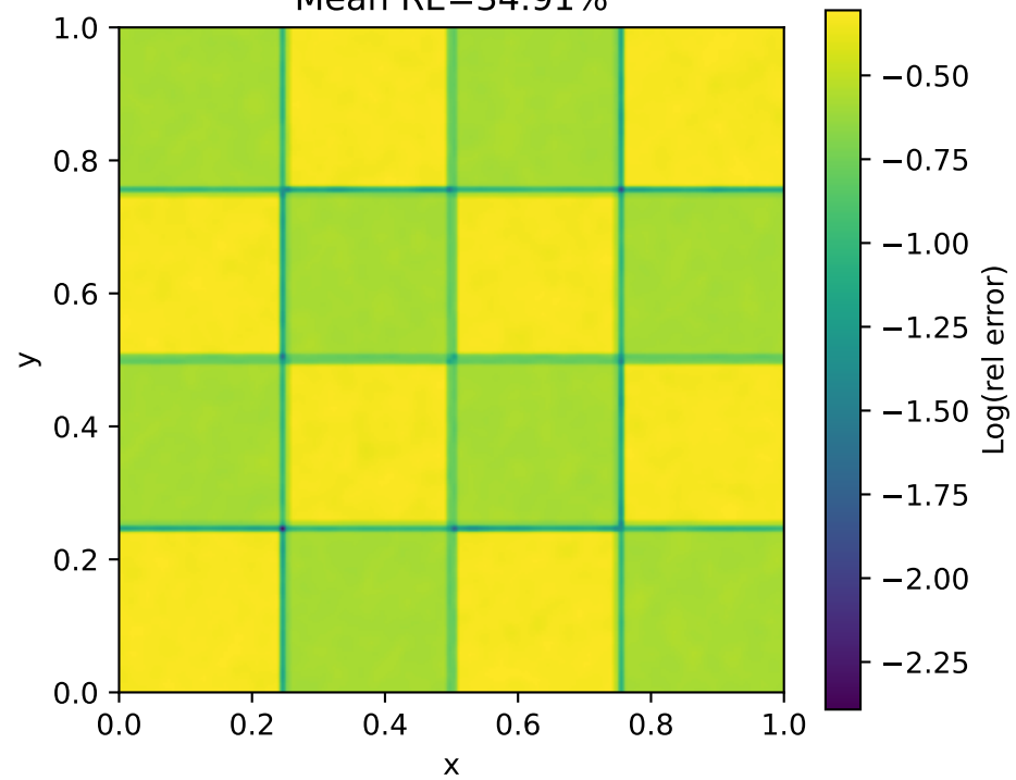
Mean RE=34.91%
