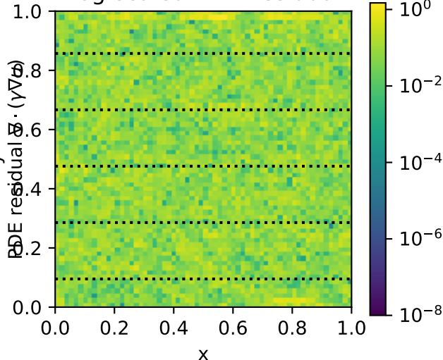
k=10 Log-scaled PDE Residual
