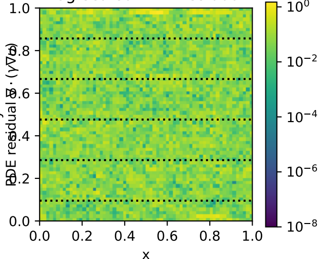
k=20 Log-scaled PDE Residual
