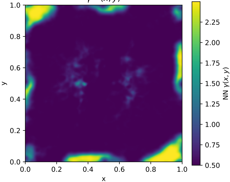
\gamma^{NN}(x, y)
