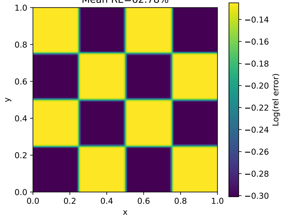
Mean RE=62.78%
