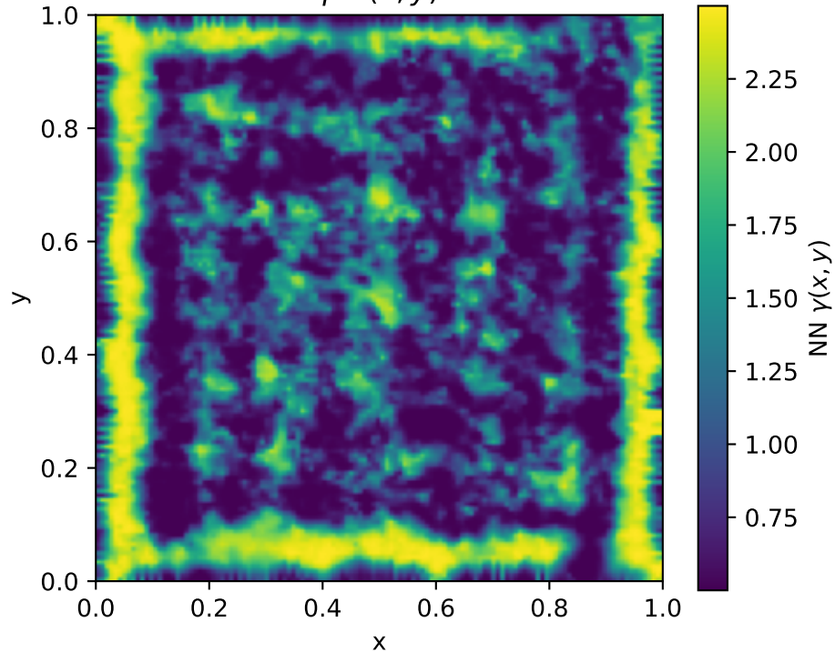
\gamma^{NN}(x, y)
