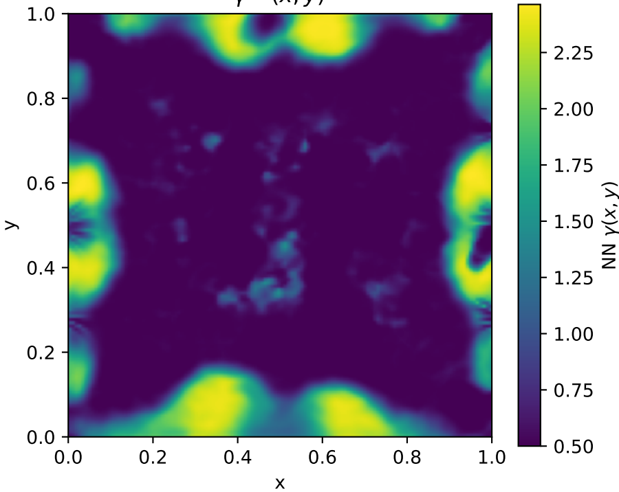
\gamma^{NN}(x, y)
