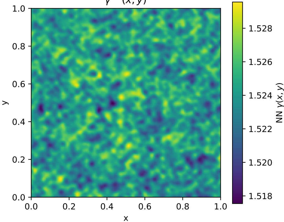
\gamma^{NN}(x, y)
