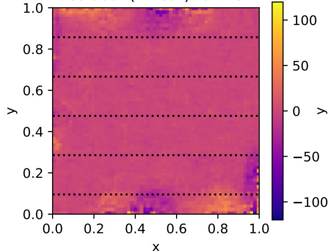
PDE Residual (Linear) for BC k=10
